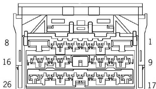
Connector Mating Side
