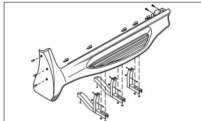
Side Step with three-bracket support per side
