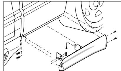
Front bed Ground Effects section
